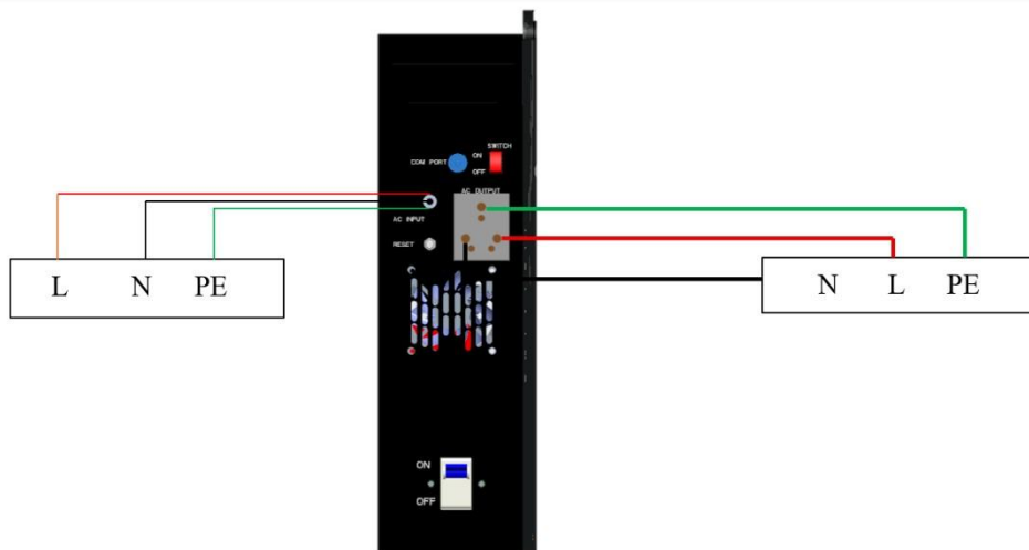
Reference wireframe diagram for AC mains input and AC output
